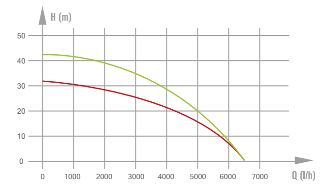
NSPQ900-3P NSPQ1100-4P NSPQ900-INOX3P NSPQ1100-INOX4P NSPQ900-INOX3Pe NSPQ1100-INOX4Pe
